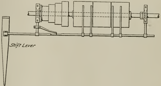
DETAILS OF AUTOMATICALLY HELD BELT SHIFTER.
